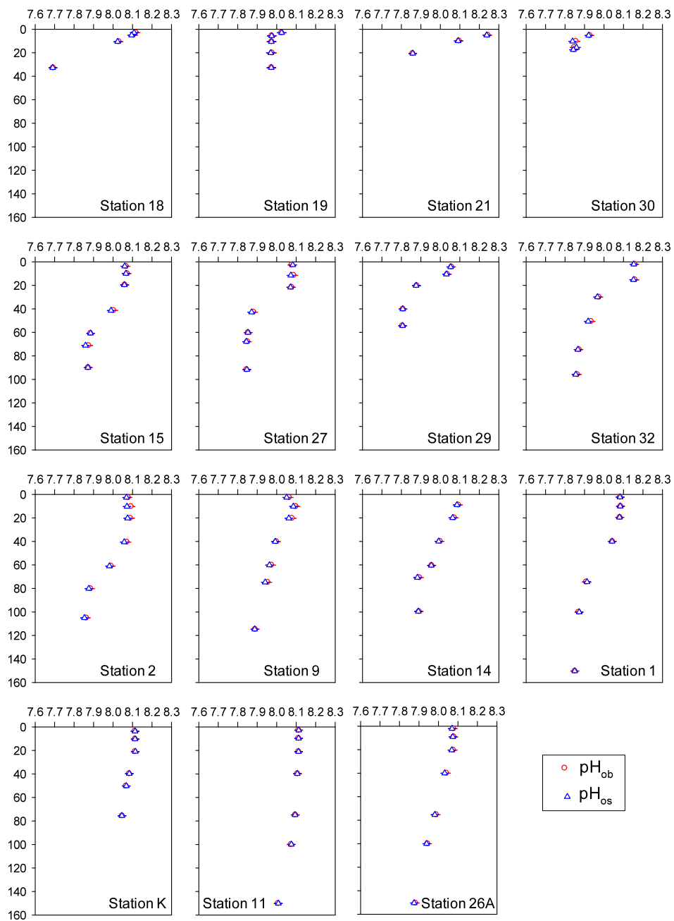
Figure 2. Depth distributions of onboard and onshore measured pH at 15 hydrographic stations on the East China Sea shelf.
