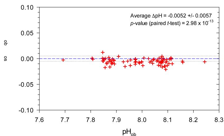
Figure 1. Difference between the onshore measured pH ( \text{pH}_{0s} ) and the onboard measured pH ( \text{pH}_{0b} ) as a function of \text{pH}_{0b} .
