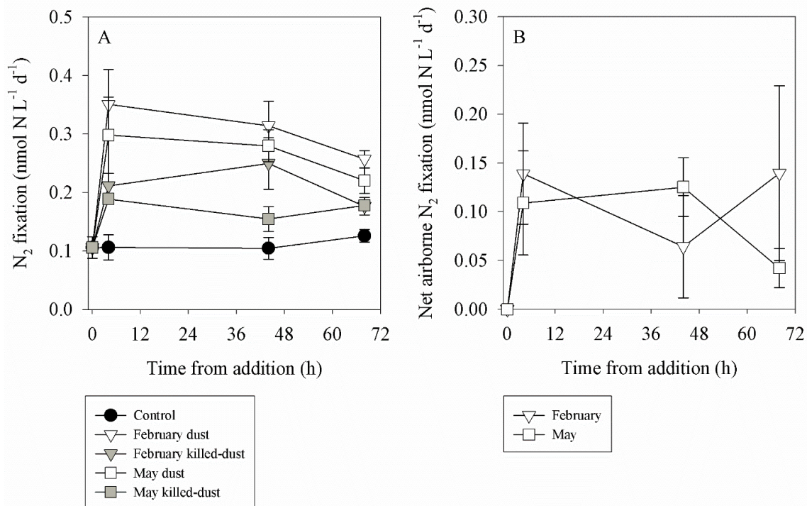
Figure: Temporal changes in volumetric N 2 fixation rates (A) and the net airborne diazotrophic activity (B) following dust additions (~0.8 mg L -1 ) to surface seawater of the Northern Red Sea during July 2017. The following treatments were performed: dust collected in February 2017 (white triangle), UV-killed February 2017 dust (gray triangle), dust collected in May 2017 (white square), UV-killed May 2017 dust (gray square) and unamended controls (black circle). Data shown is the averages of 3 replicate mesocosms per treatment and their corresponding standard deviation. Note the different Y-axis. The net airborne diazotrophic contribution was calculated by subtracting the 'killed-dust' rates from the rates measured in the 'dust' treatments.
